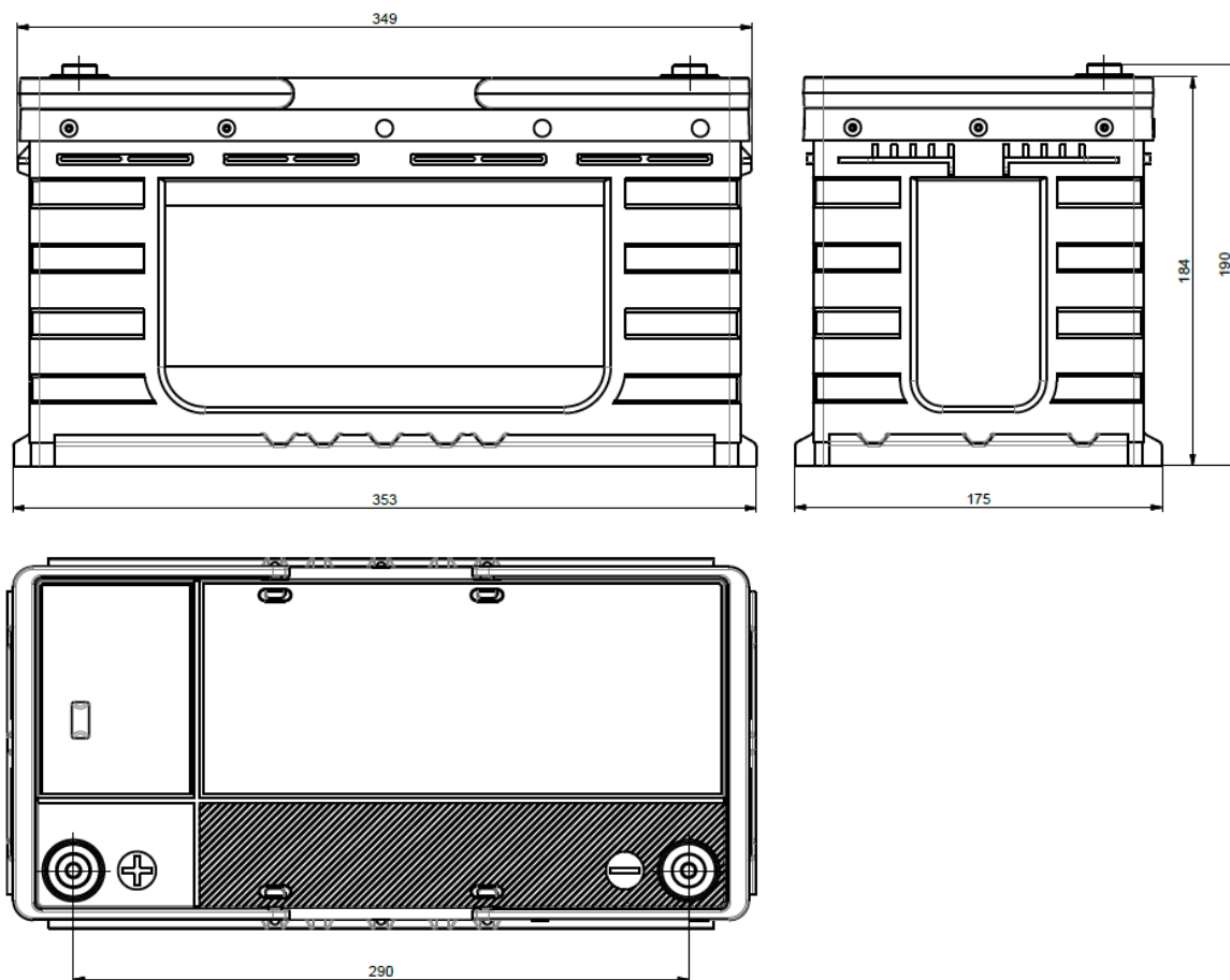
Figure 1. Dimensions of the lithium-ion battery with M6 screw threads
