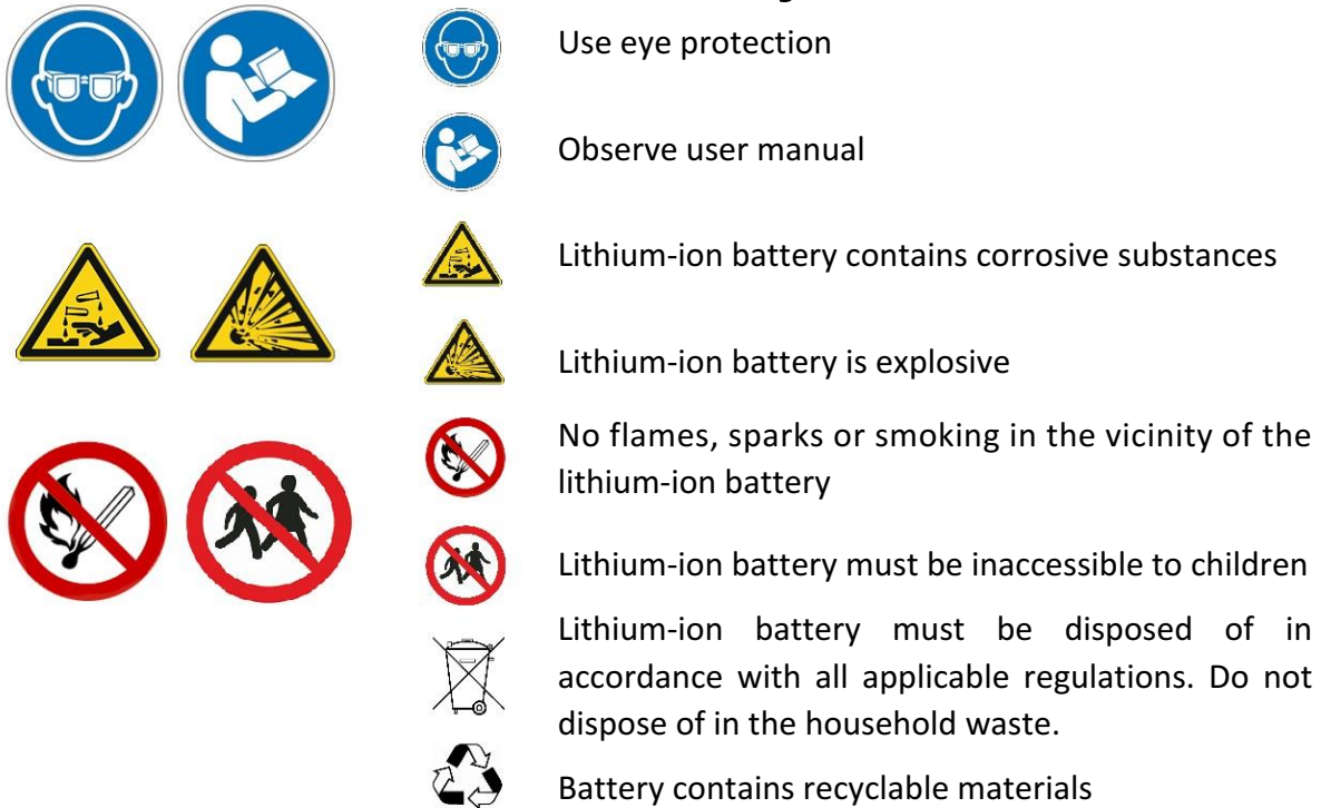
Figure 4. Safety symbols
